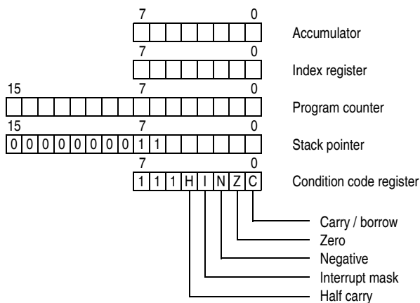
Figure 10-1 Programming model
