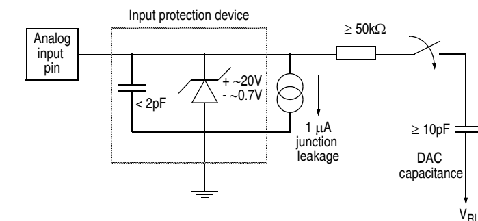
Figure 8-2 Electrical model of an A/D input pin
