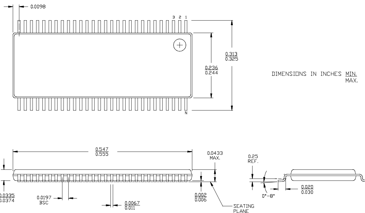
56-Lead Thin Shrunk Small Outline Package Z56
