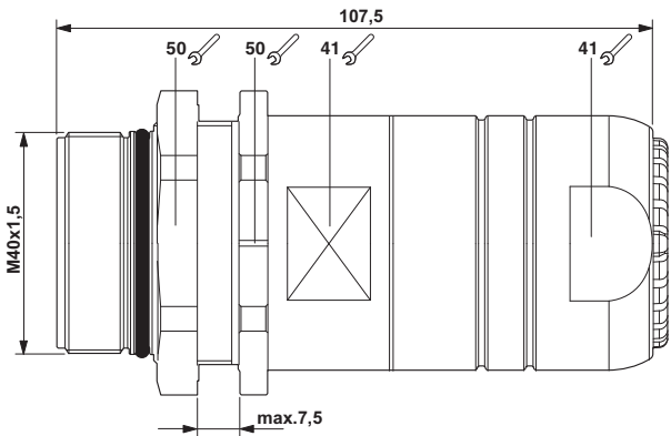
Dimensioned drawing
