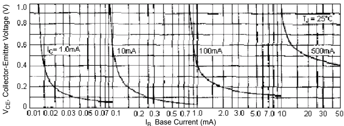
DC Current Gain
