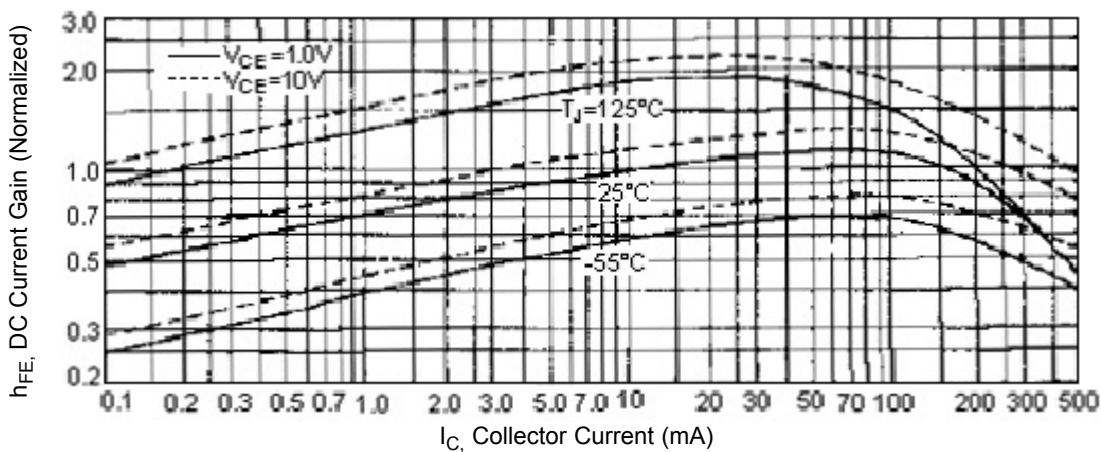
DC Current Gain
