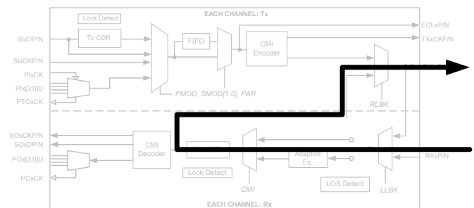
Figure 7: Remote (Analog) Loopback
