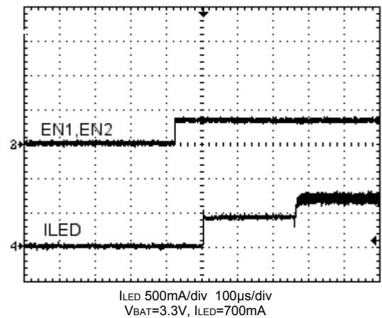
Figure 7 – Startup of AS3685A -- ILED Current
