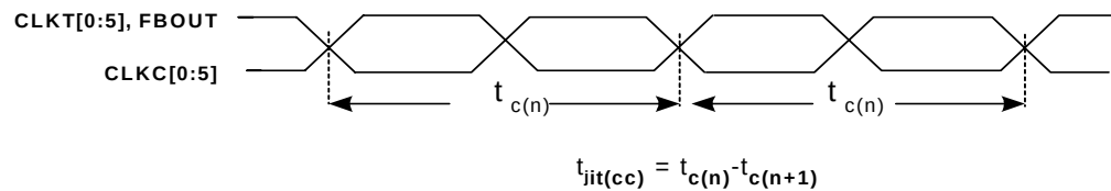
Figure 6. Cycle-to-Cycle Jitter
