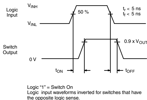
Figure 1. Switching Time
