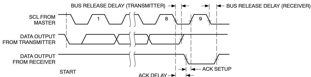
Figure 9. Acknowledge Timing
