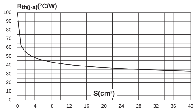
Figure 11. DPAK thermal resistance junction to ambient versus copper surface under tab (printed circuit board FR4, copper thickness: 35 μm)
