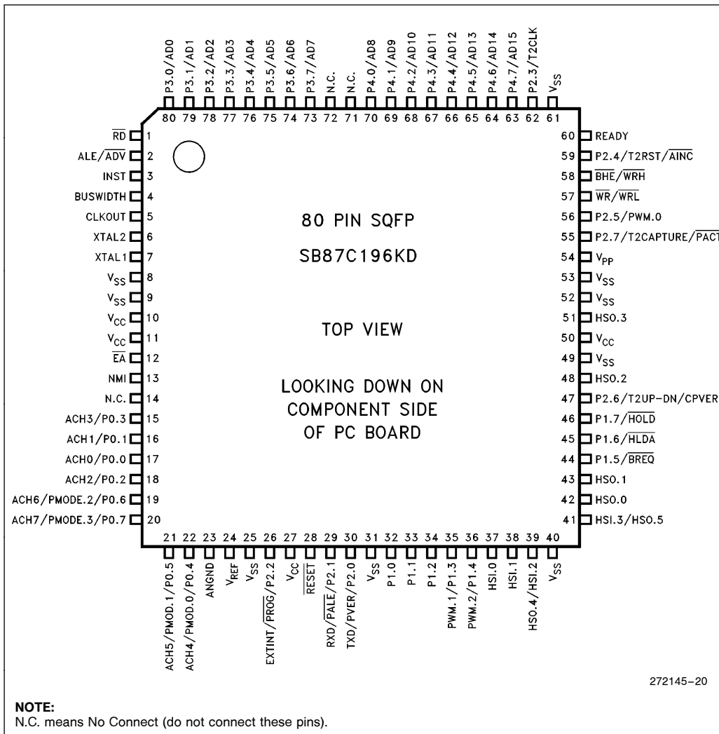
Figure 6. 80-Pin SQFP Package
