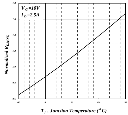
Fig 4. Normalized On-Resistance
