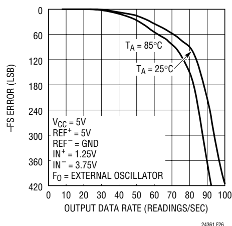
Figure 26. -FS Error vs Output Data Rate and Temperature
