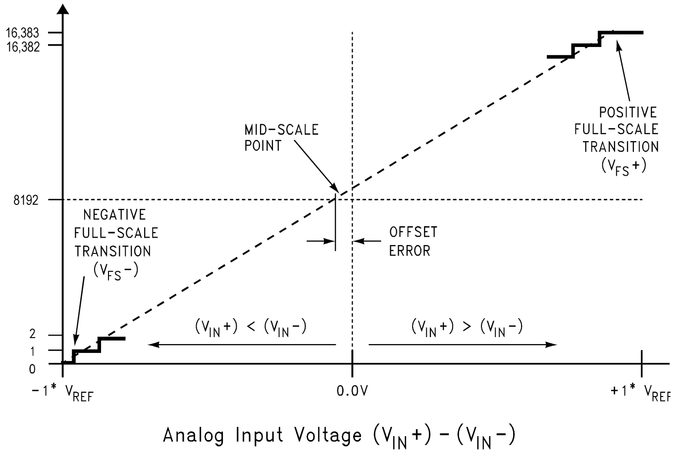
Figure 2. Transfer Characteristic
