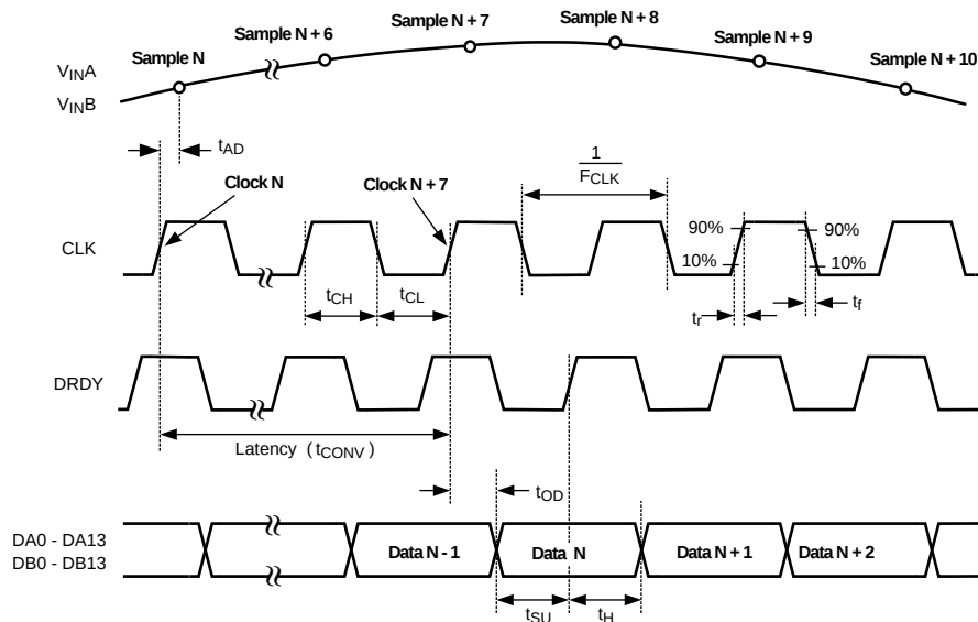
Figure 1. Output Timing
