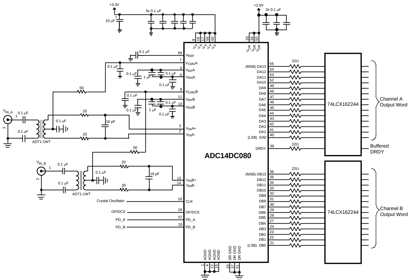
Figure 21. Application Circuit
