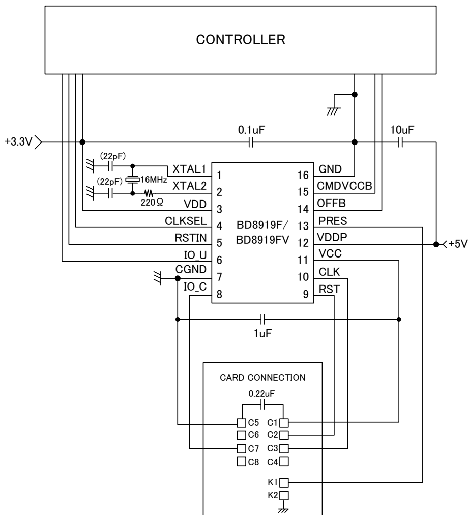
BD8919F/FV application examples
