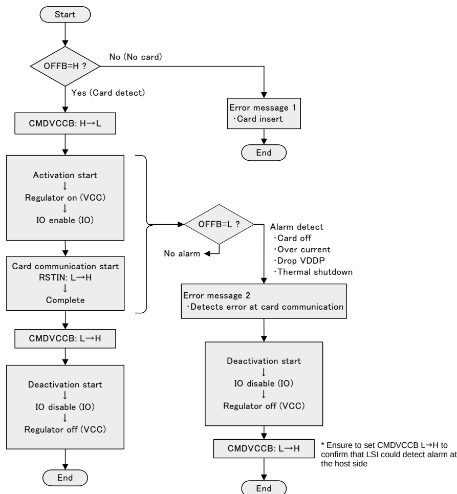
Fig. 7 An example of software control
