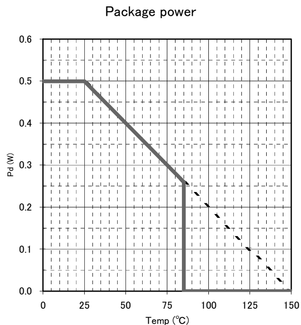
Fig. 1.2 BD8918FV/BD8919FV Power Dissipation
