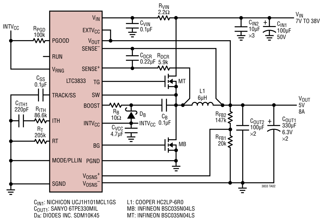
5V, 8A, 200kHz High Efficient Step-Down Converter
