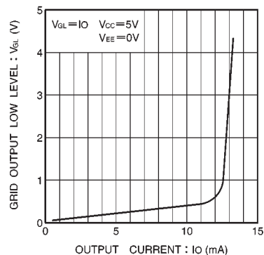
Fig. 8 Grid low level output vs. output current
