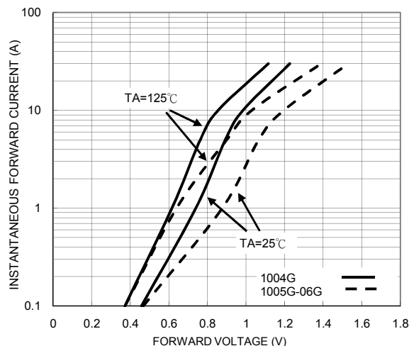
FIG. 4 TYPICAL FORWARD CHARACTERISRICS
