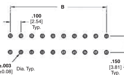
Recommended PC Board Hole Layout for Top Entry
