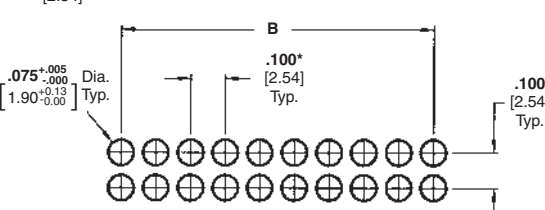
Recommended PC Board Hole Layout for Bottom Entry or Pass Through Applications
