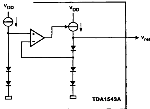
(b) output pin V_{ref} .
