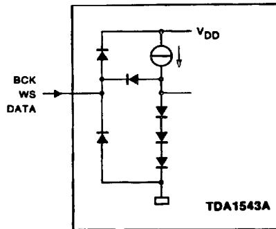
(a) input pins BCK, WS and DATA.
