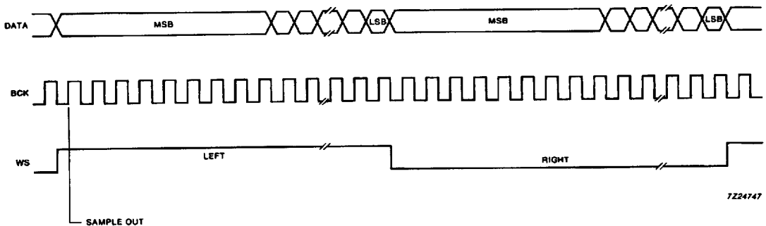
Fig.5 Format of input signals.
