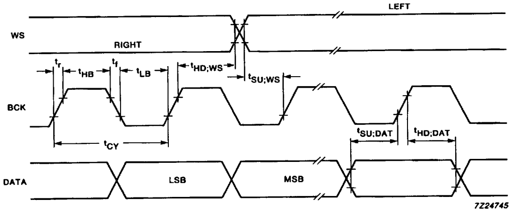
Fig.4 Format of input signals (Japanese format).
