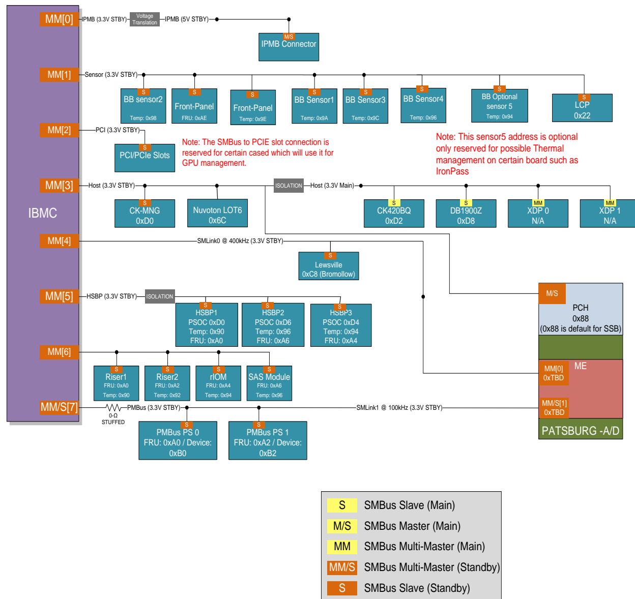
Figure 14. Server Management Bus (SMBUS*) Block Diagram
