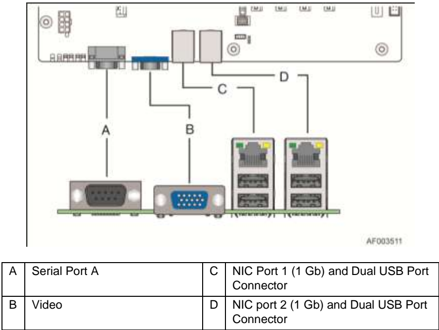
Figure 10. Intel® Server Board S1200BT Rear I/O Layout
