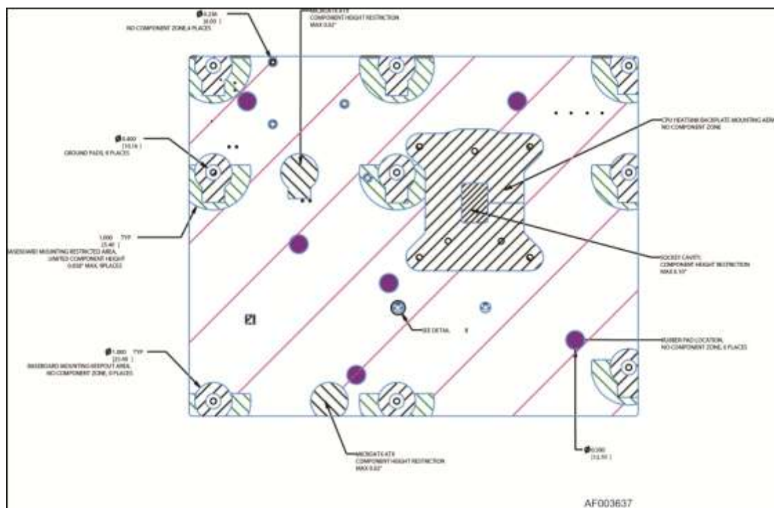
Figure 9. Intel® Server Board S1200BTL/S1200BTLRM – Secondary Side Keepout Zone
