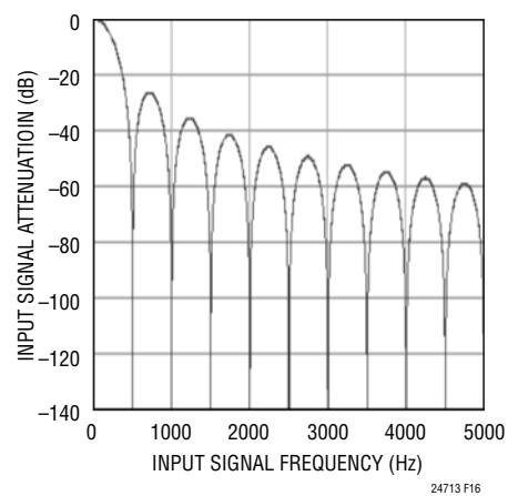
Figure 16. LTC2473 Input Signal Attenuation vs Frequency (208sps Mode)
