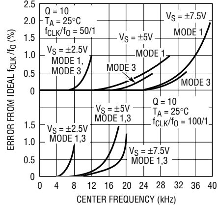
f_{CLK}/f_0 vs f_0
