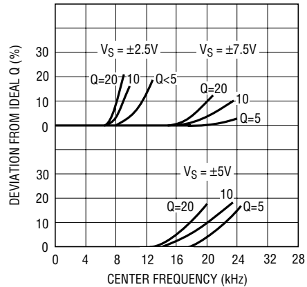
Mode 1: ( f_{CLK}/f_0 ) = 100:1
