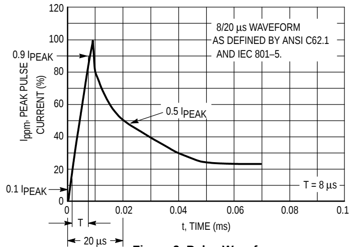
Figure 9. Pulse Waveform
