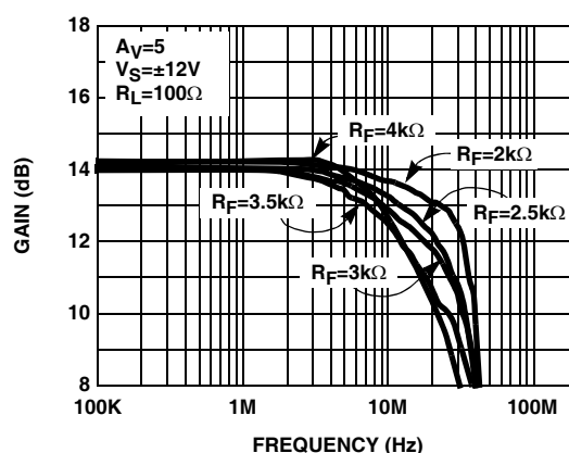
FIGURE 4. DIFFERENTIAL FREQUENCY RESPONSE vs R_F (2/3 POWER MODE)
