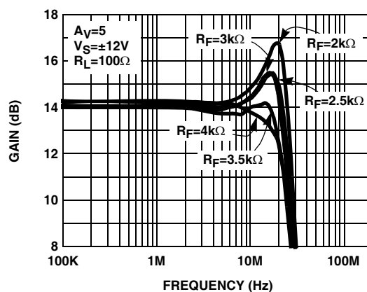
FIGURE 2. DIFFERENTIAL FREQUENCY RESPONSE vs R_F (1/3 POWER MODE)
