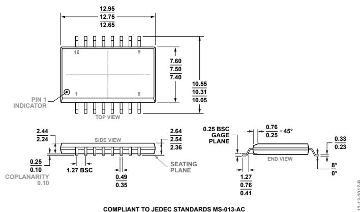
Figure 19. 16-Lead Standard Small Outline Package, with Increased Creepage [SOIC_IC] Wide Body (RI-16-2) Dimensions shown in millimeters
