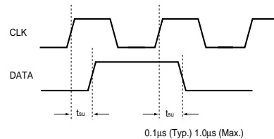
Fig. 6 Clock rising edge and data relationship (setup time)
