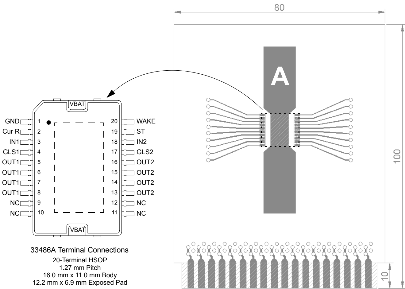
Figure 31. Thermal Test Board
