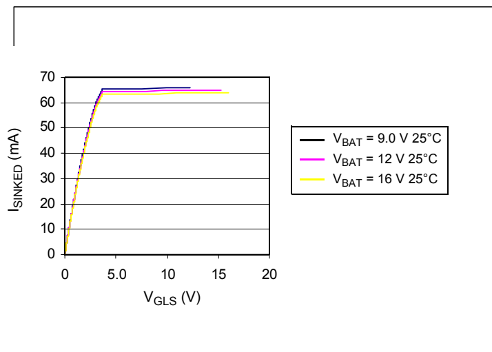
Figure 14. Gate Low-Side (GLS) Sinked Current Capability (High-Speed Mode)
