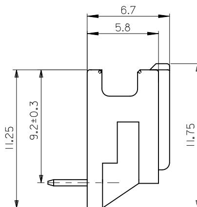
SECT. X-X
