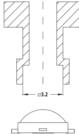
Figure 24. Recommended pick and place nozzle tip. Inner diameter = 3.2 mm.
