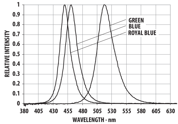
Figure 12. Relative Intensity vs. Wavelength for Blue, Royal Blue and Green
