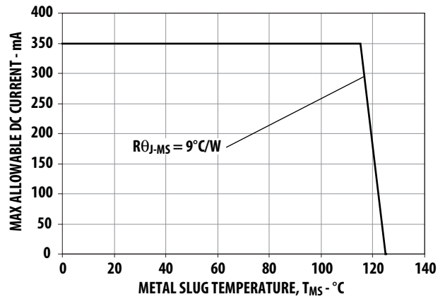
Figure 10. Maximum Forward Current vs. Ambient Temperature. Derated based on T_{JMAX} = 125^\circ\text{C} , R_{\theta MS} = 9^\circ\text{C/W}
