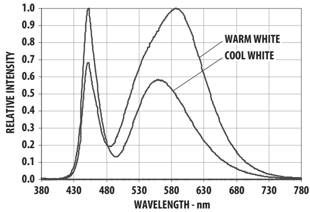
Figure 11. Relative Intensity vs. Wavelength for Cool and Warm White
