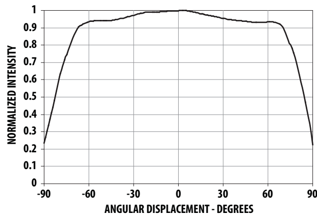
Figure 15. Radiation Pattern for Blue, Royal Blue and Green
