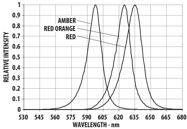
Figure 1. Relative Intensity vs. Wavelength for Red, Red-Orange and Amber
