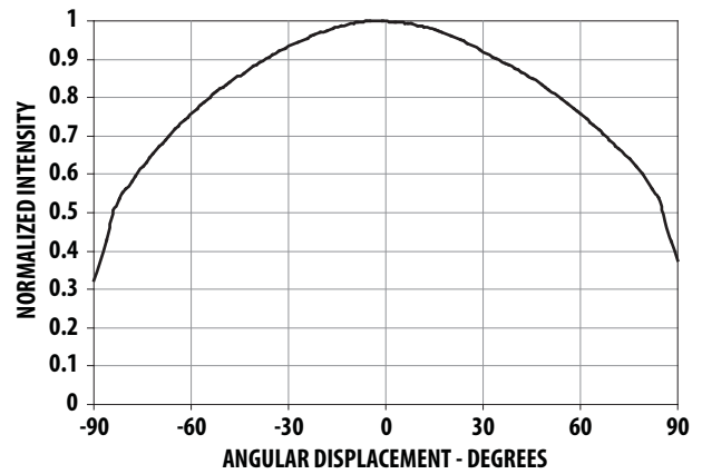
Figure 4. Radiation Pattern for Red, Red Orange and Amber
