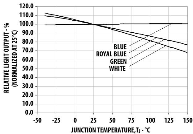
Figure 19. Relative Light Output vs. Junction Temperature
