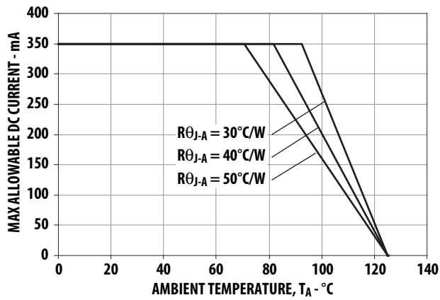
Figure 9. Maximum Forward Current vs. Ambient Temperature. Derated based on T_{JMAX} = 125^\circ\text{C} , R_{\theta JA} = 30^\circ\text{C/W} , 40^\circ\text{C/W} and 50^\circ\text{C/W}
