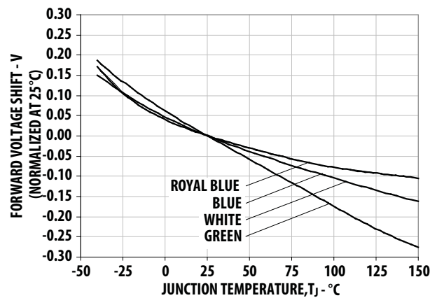
Figure 20. Forward Voltage Shift vs. Junction Temperature
