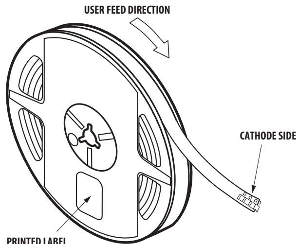
Figure 31. Reeling Orientation
