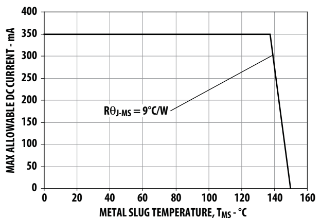
Figure 22. Maximum Forward Current vs. Metal Slug Temperature. Derated based on T_{JMAX} = 150^\circ\text{C} , R\theta_{J-MS} = 9^\circ\text{C/W} .
