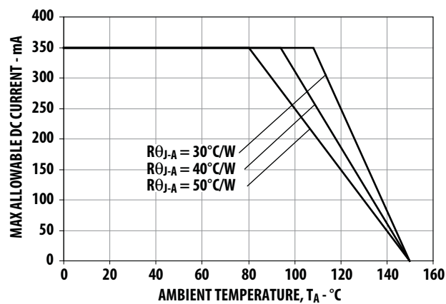
Figure 21. Maximum Forward Current vs. Ambient Temperature. Derated based on T_{JMAX} = 150^\circ\text{C} , R\theta_{J-A} = 30^\circ\text{C/W} , 40^\circ\text{C/W} and 50^\circ\text{C/W}
