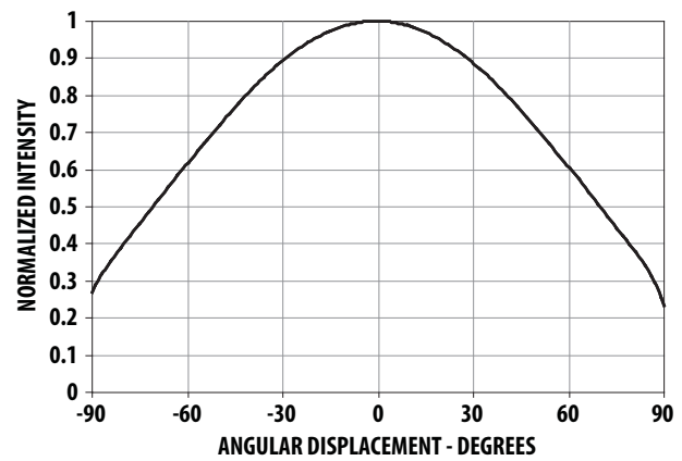
Figure 16. Radiation Pattern for Cool White, Neutral White and Warm White
