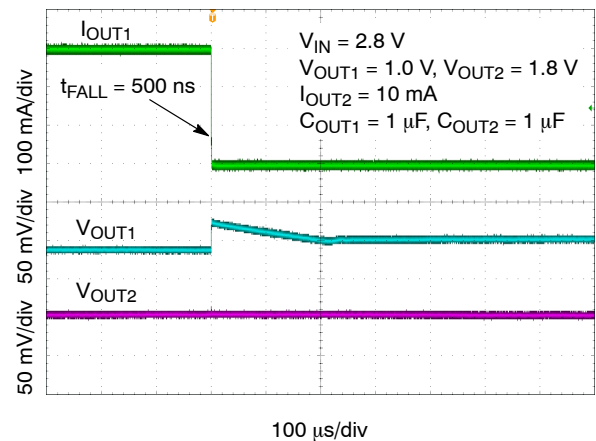
Figure 41. Load Transient Response – 1.0 V – Falling Edge, I_{OUT1} = 300 \text{ mA} to 100 \mu\text{A}
