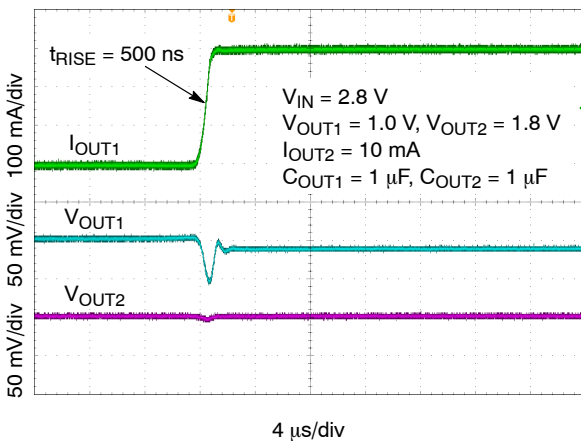
Figure 40. Load Transient Response – 1.0 V – Rising Edge, I_{OUT1} = 100 \mu\text{A} to 300 \text{ mA}
