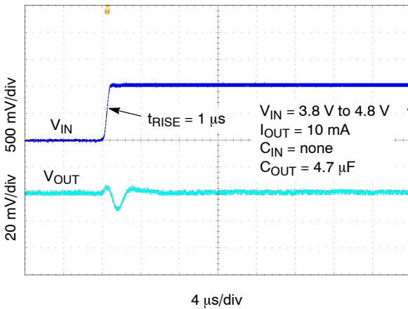
Figure 38. Line Transient Response– Rising Edge, V_{OUT} = 3.3 \text{ V} , I_{OUT} = 10 \text{ mA} , C_{OUT} = 4.7 \mu\text{F}
