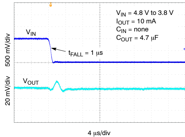
Figure 39. Line Transient Response– Falling Edge, V_{OUT} = 3.3 \text{ V} , I_{OUT} = 10 \text{ mA} , C_{OUT} = 4.7 \mu\text{F}
