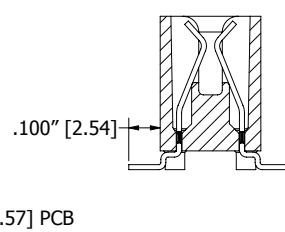
SURFACE MOUNT (YF)
