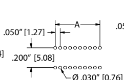
PCB LAYOUT (YS)
