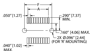
PCB LAYOUT (YF)
