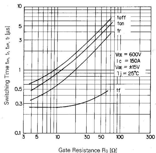
Switching Time-Gate Resistance
