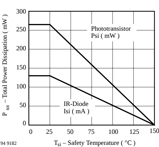
Figure 1. Derating diagram
