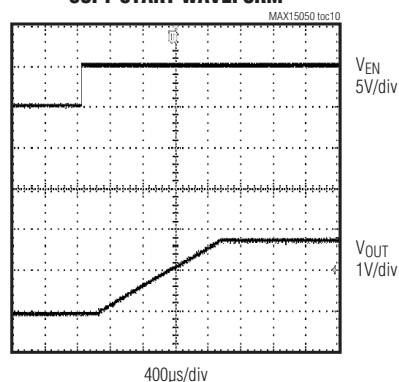
SOFT-START WAVEFORM
