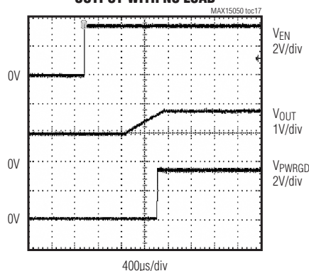
STARTING INTO PREBIASED OUTPUT WITH NO LOAD
