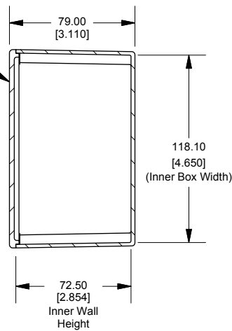
SECTION A-A End View of Assembly
