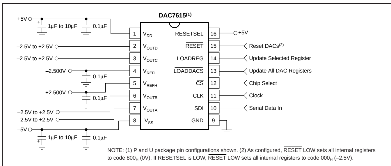
FIGURE 2. Basic Dual-Supply Operation of the DAC7615.
