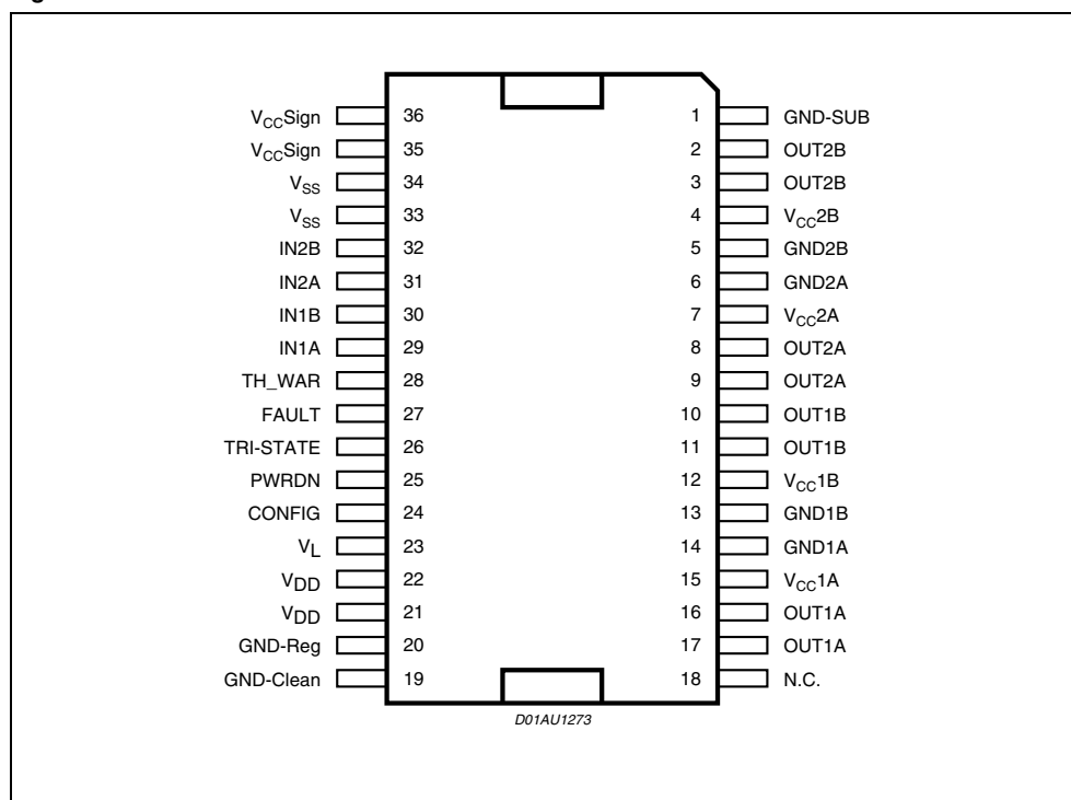
Figure 3. Pin Connection
