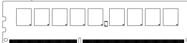
Figure 2: 240-Pin UDIMM (MO-269 R/C D1)
