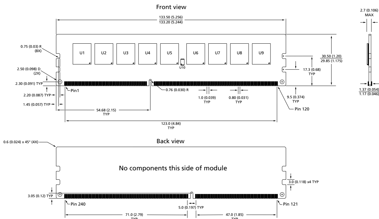
Figure 5: 240-Pin DDR3 UDIMM (PCB 1568)
