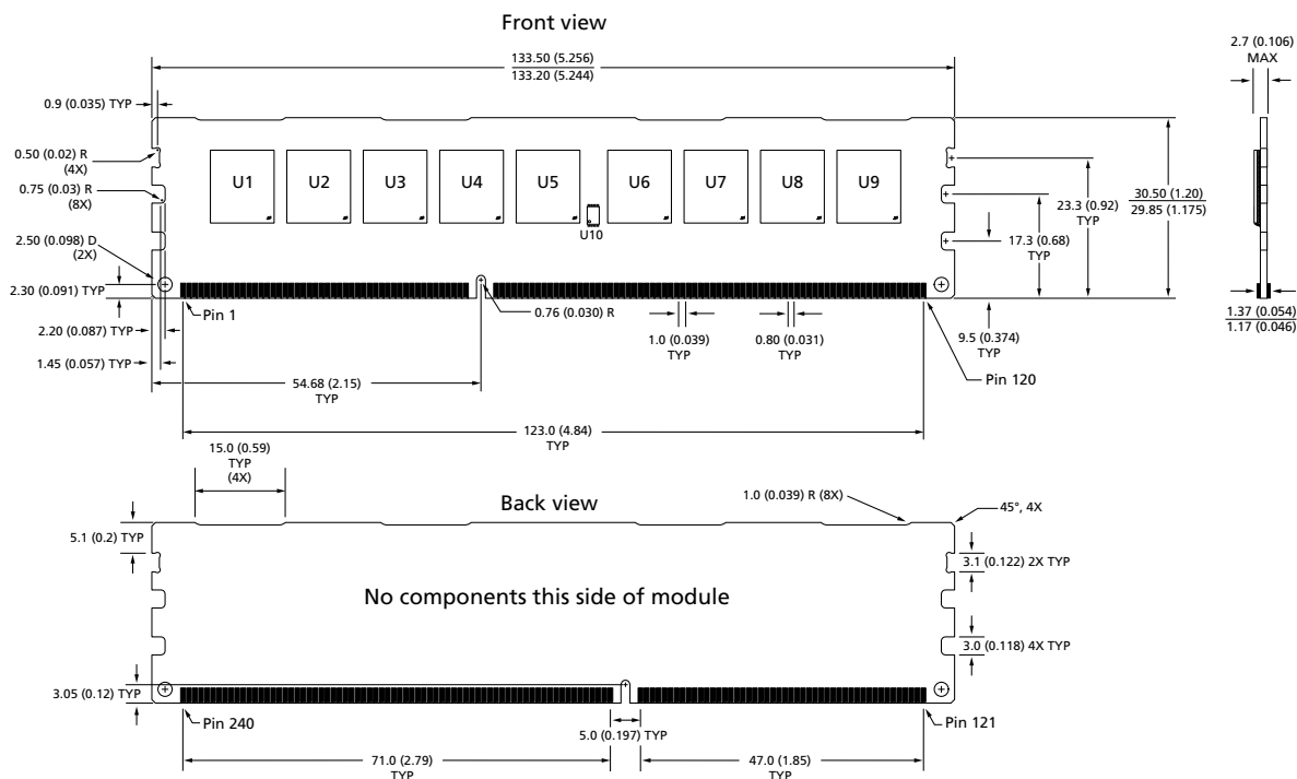
Figure 4: 240-Pin DDR3 UDIMM (PCB 1125)
