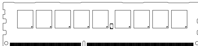
Figure 2: 240-Pin UDIMM (MO-269 R/C D1)
