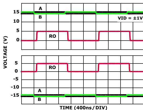
FIGURE 20. \pm 15V RECEIVER PERFORMANCE (ISL31475E)
