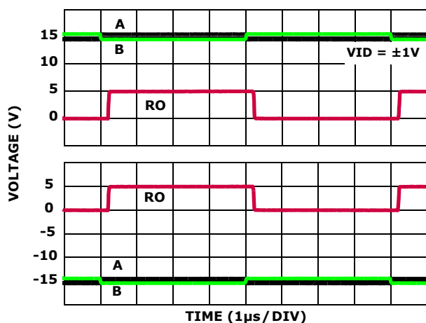
FIGURE 19. \pm 15V RECEIVER PERFORMANCE (ISL31470E, ISL31472E)
