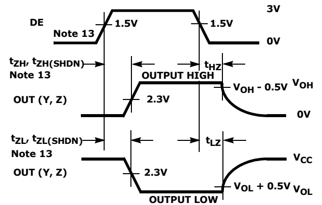
FIGURE 3A. TEST CIRCUIT FIGURE 3. DRIVER ENABLE AND DISABLE TIMES
