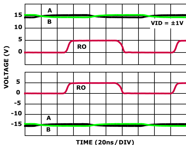
FIGURE 21. \pm 15V RECEIVER PERFORMANCE (ISL31478E)
