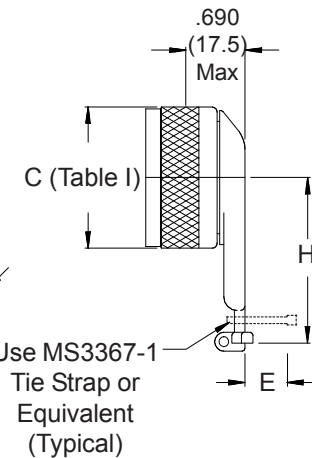
90° ROTATABLE COUPLING
