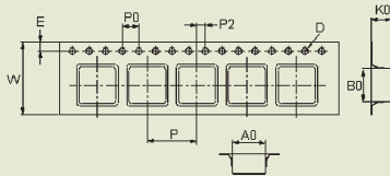
Tape Dimensions
