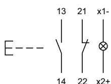
10 Illuminated pushbutton actuator page 7 | Mushroom-head pushbutton actuator page 8
