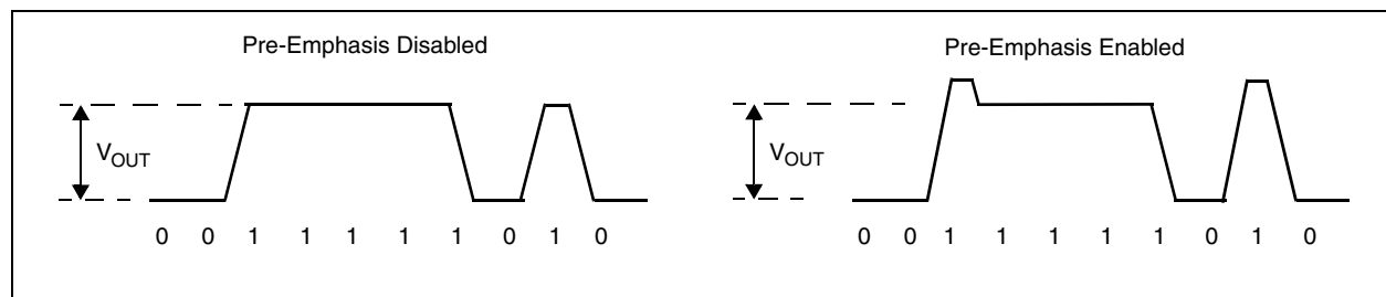
Figure 5. Pre-Emphasis Diagram
