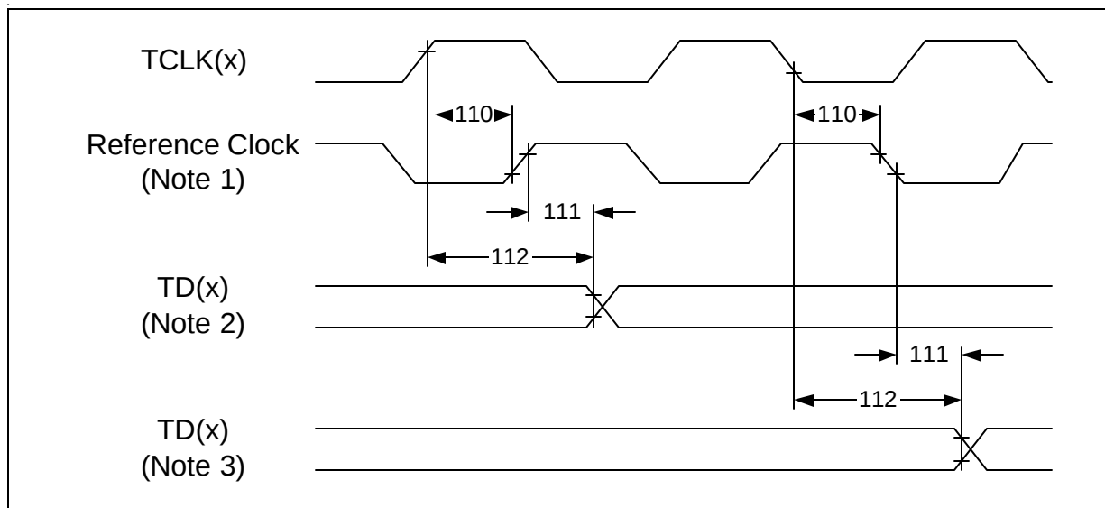
Figure 9-21 Transmit Cycle Timing
