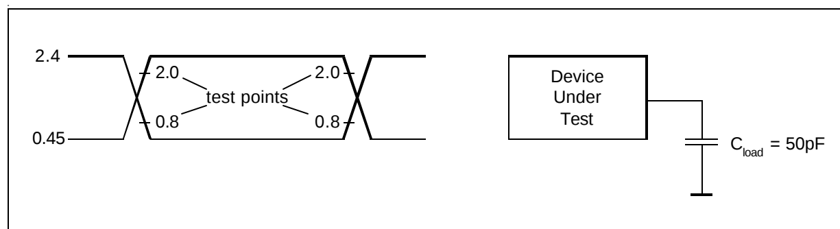
Figure 9-1 Input/Output Waveform for AC Tests
