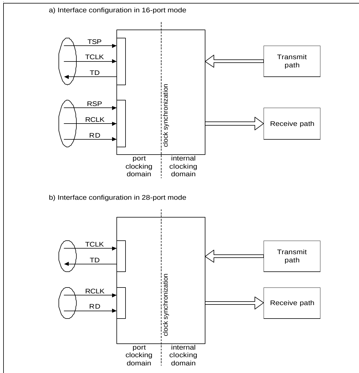
Figure 4-1 Port Configuration
