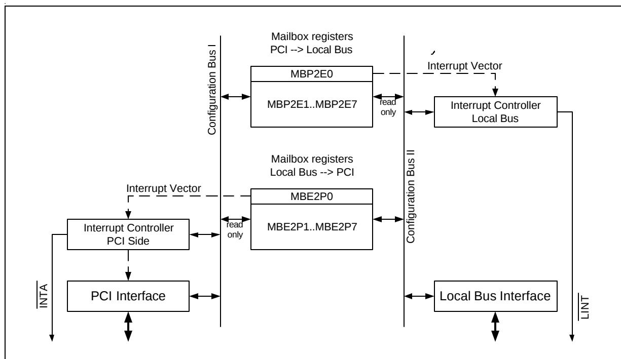
Figure 4-12 Mailbox Structure
