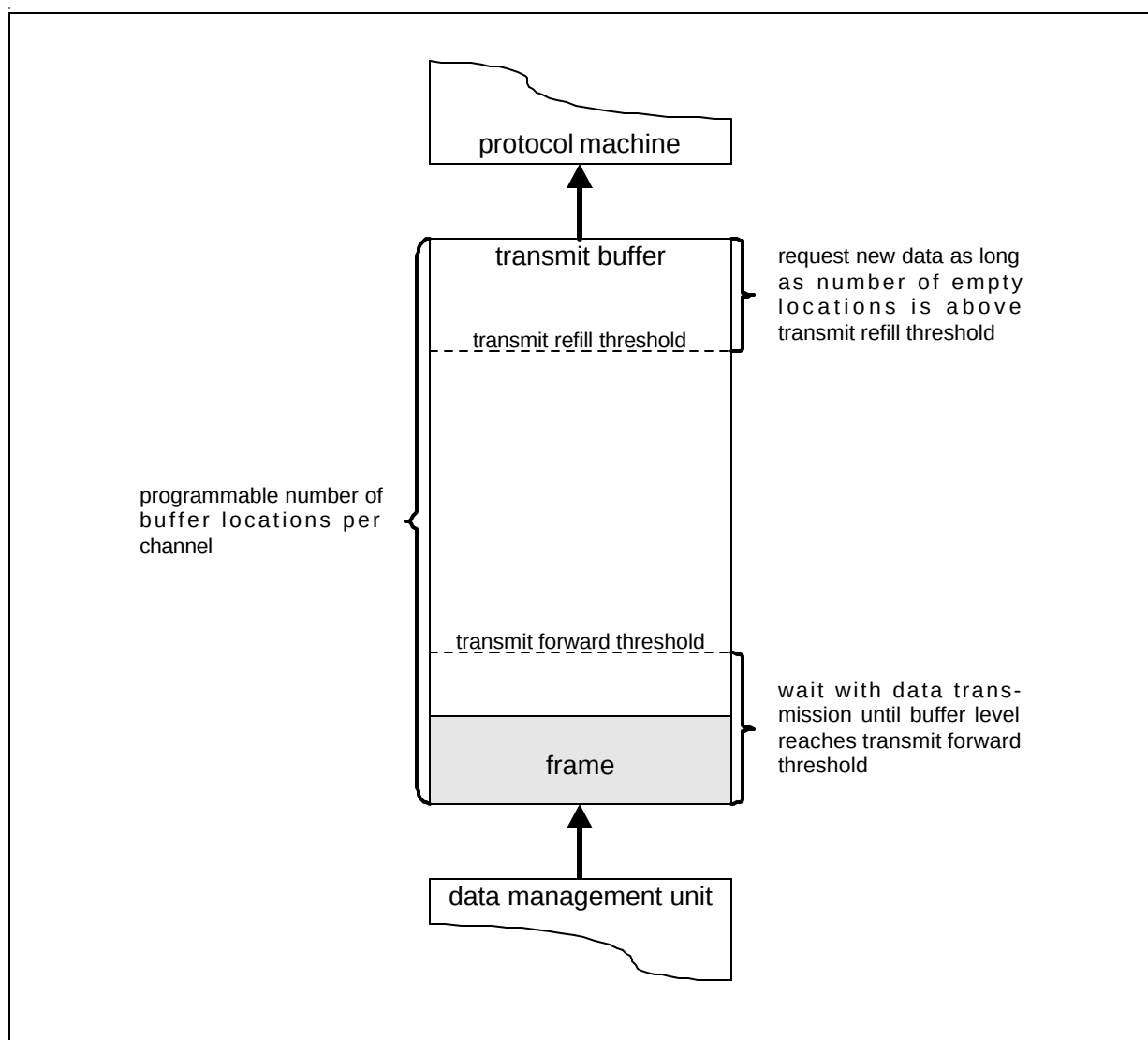
Figure 4-9 Transmit Buffer Thresholds
