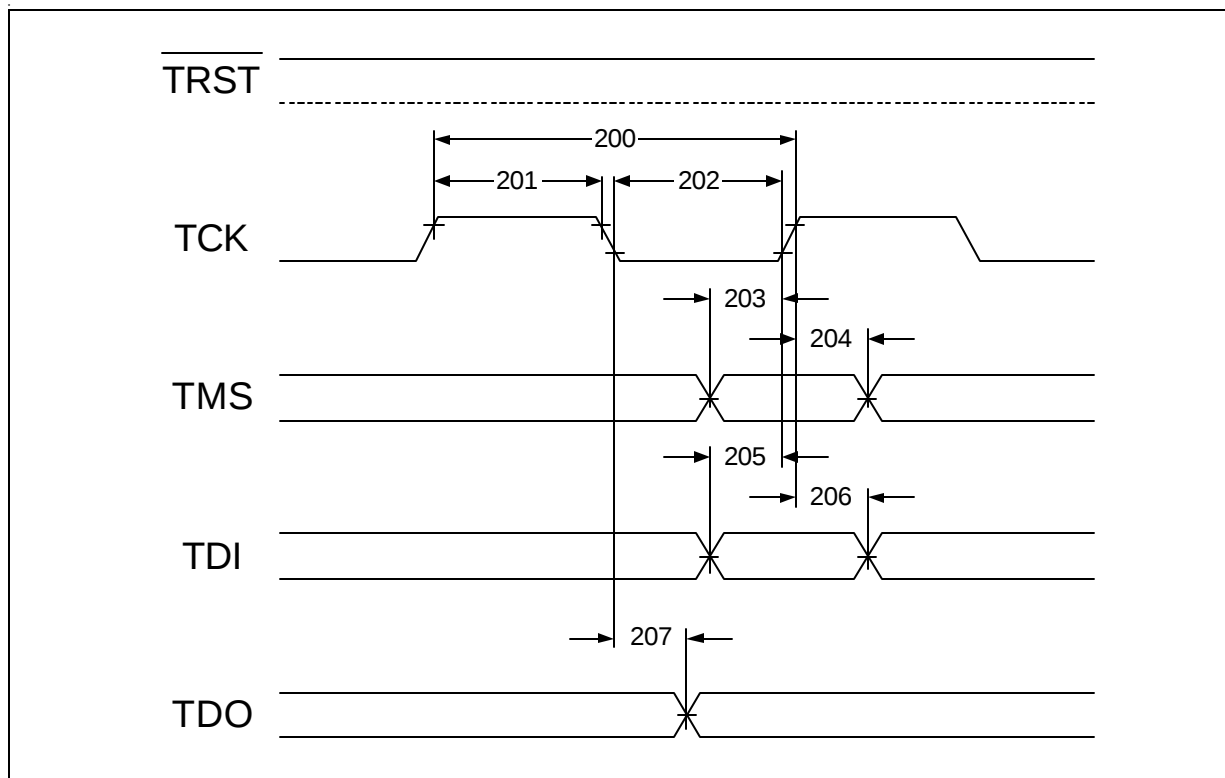
Figure 9-25 JTAG Interface Timing
