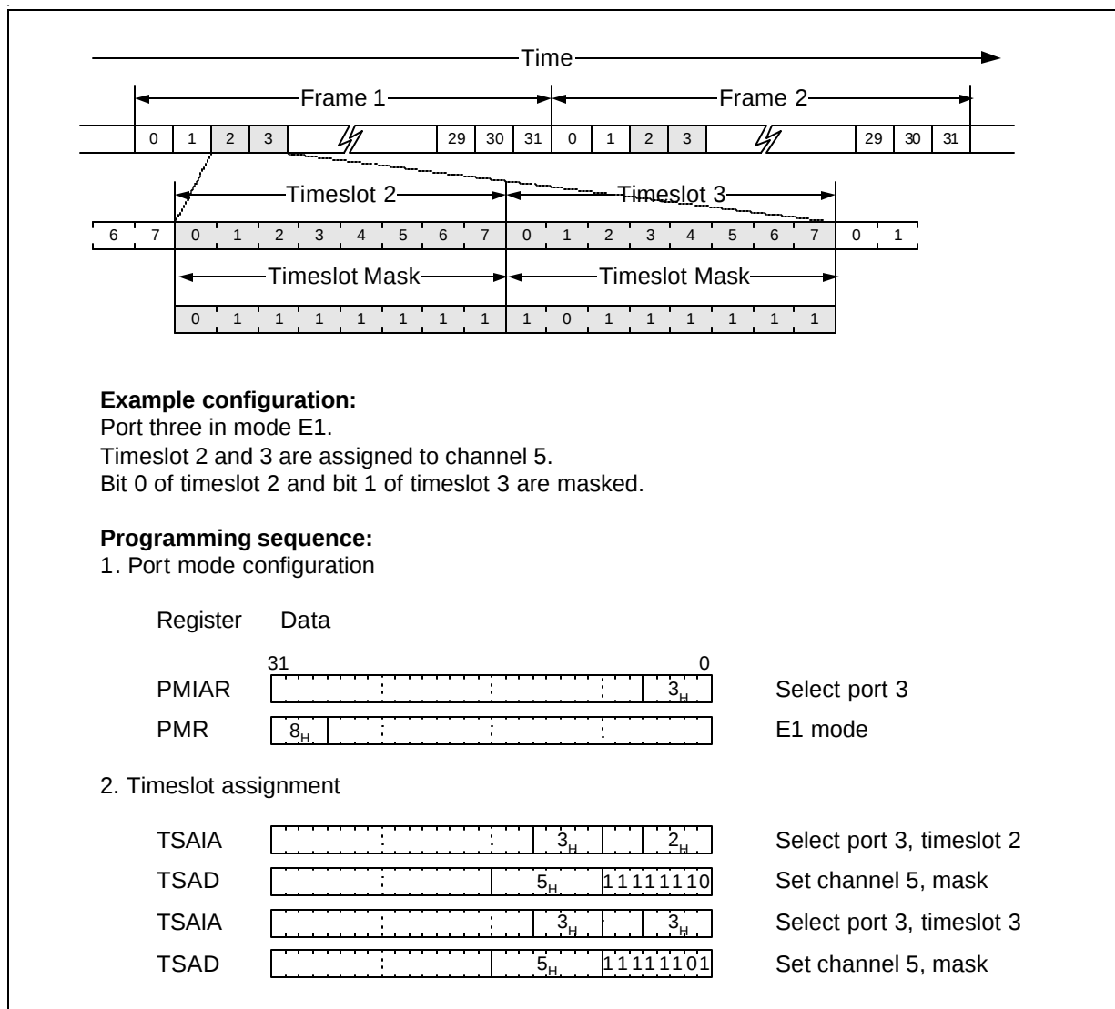
Figure 4-6 Time slot Assignment in Channelized Modes
