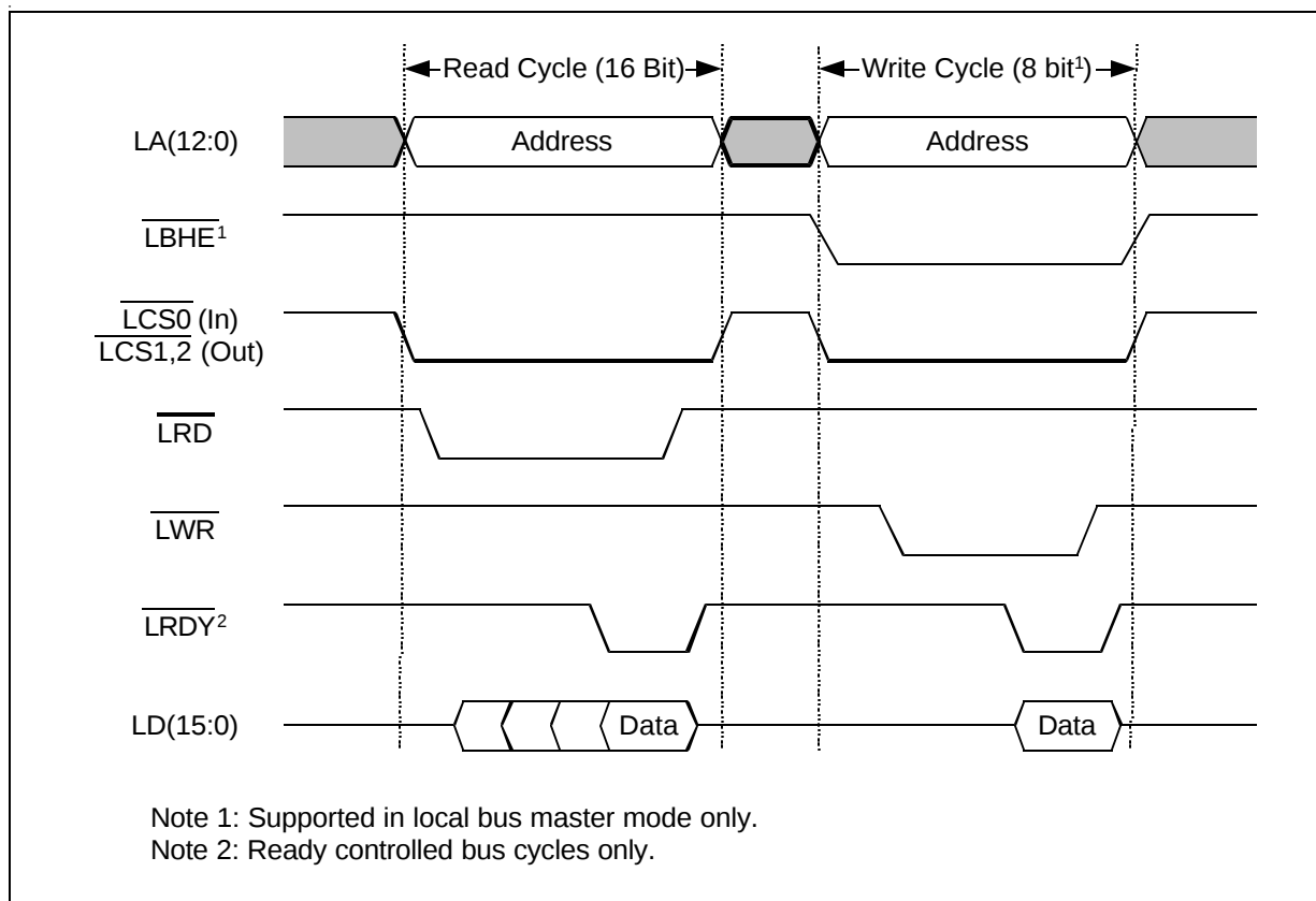
Figure 5-5 Intel Bus Mode
