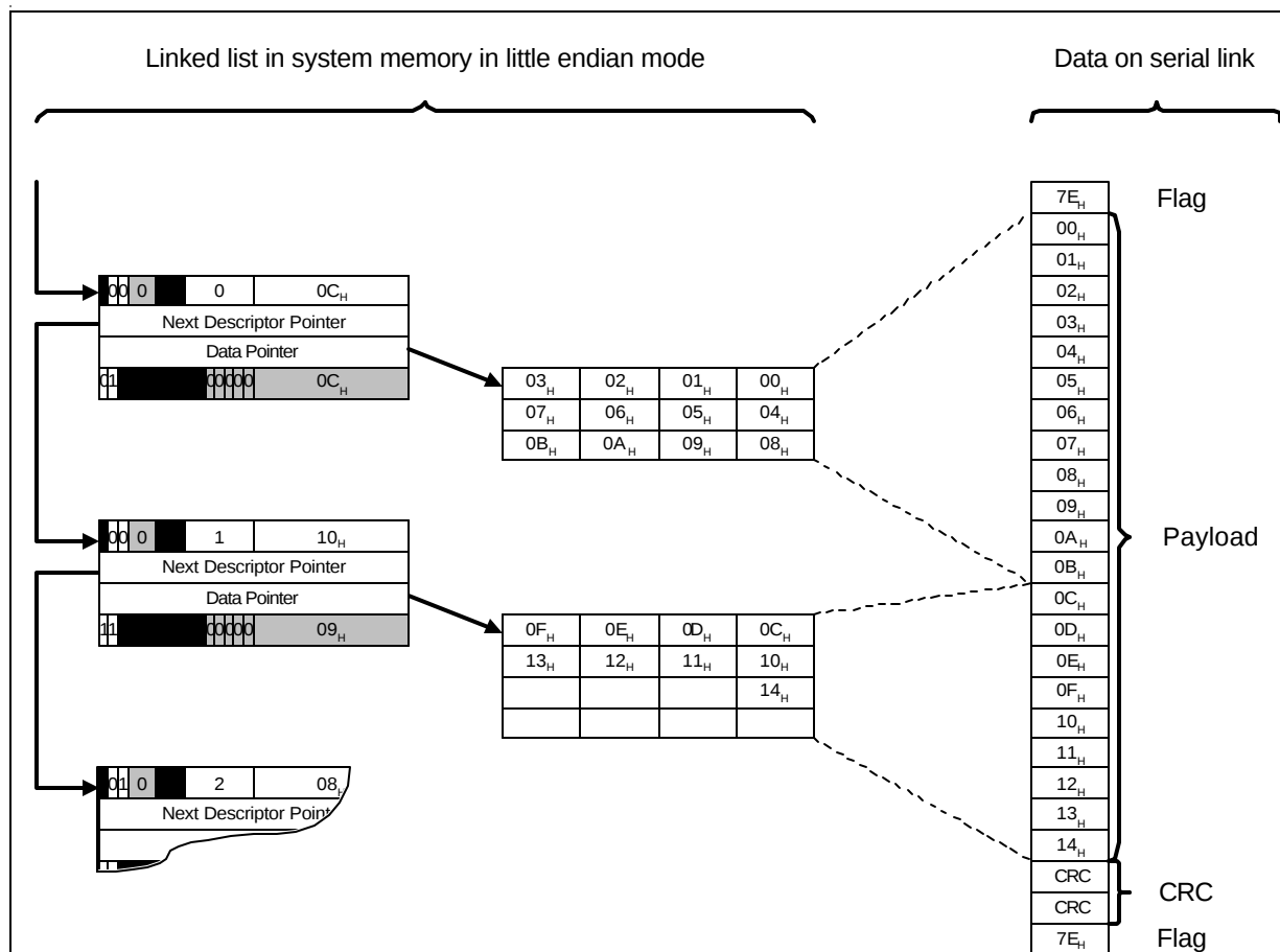
Figure 4-7 Descriptor Structure
