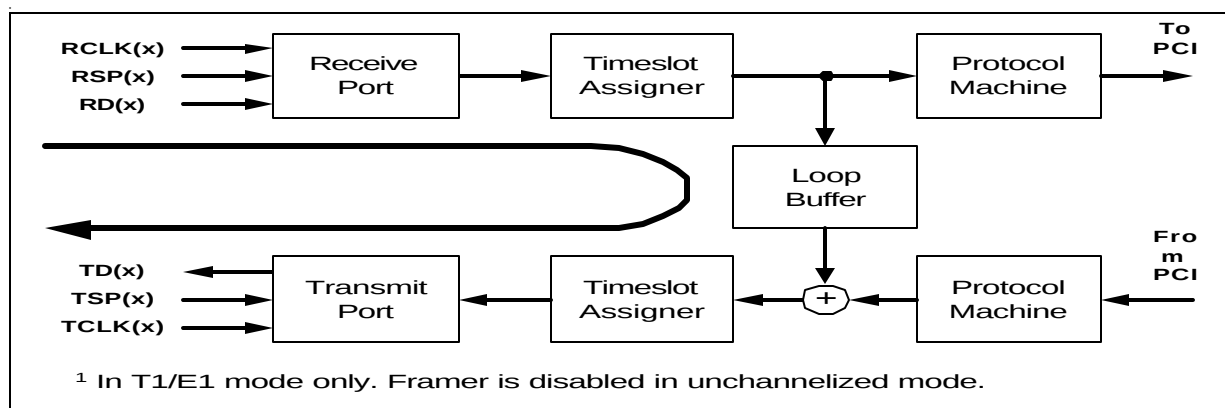
Figure 4-3 Remote Payload Loop
