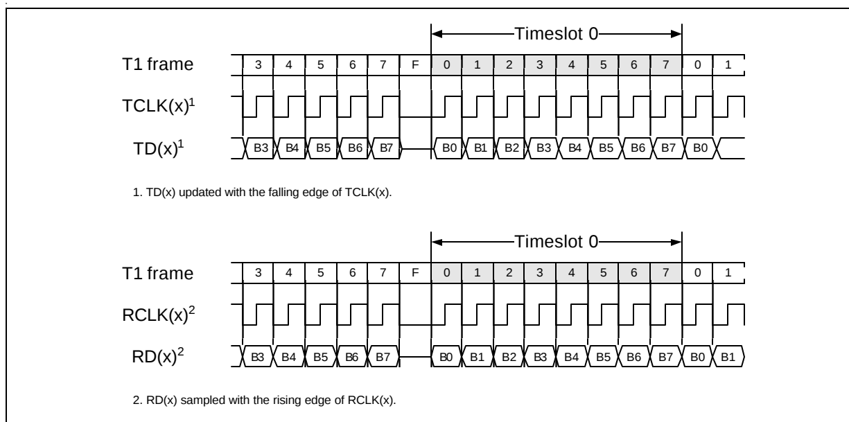
Figure 5-13 T1-mode Interface Timing in 28-port Mode
