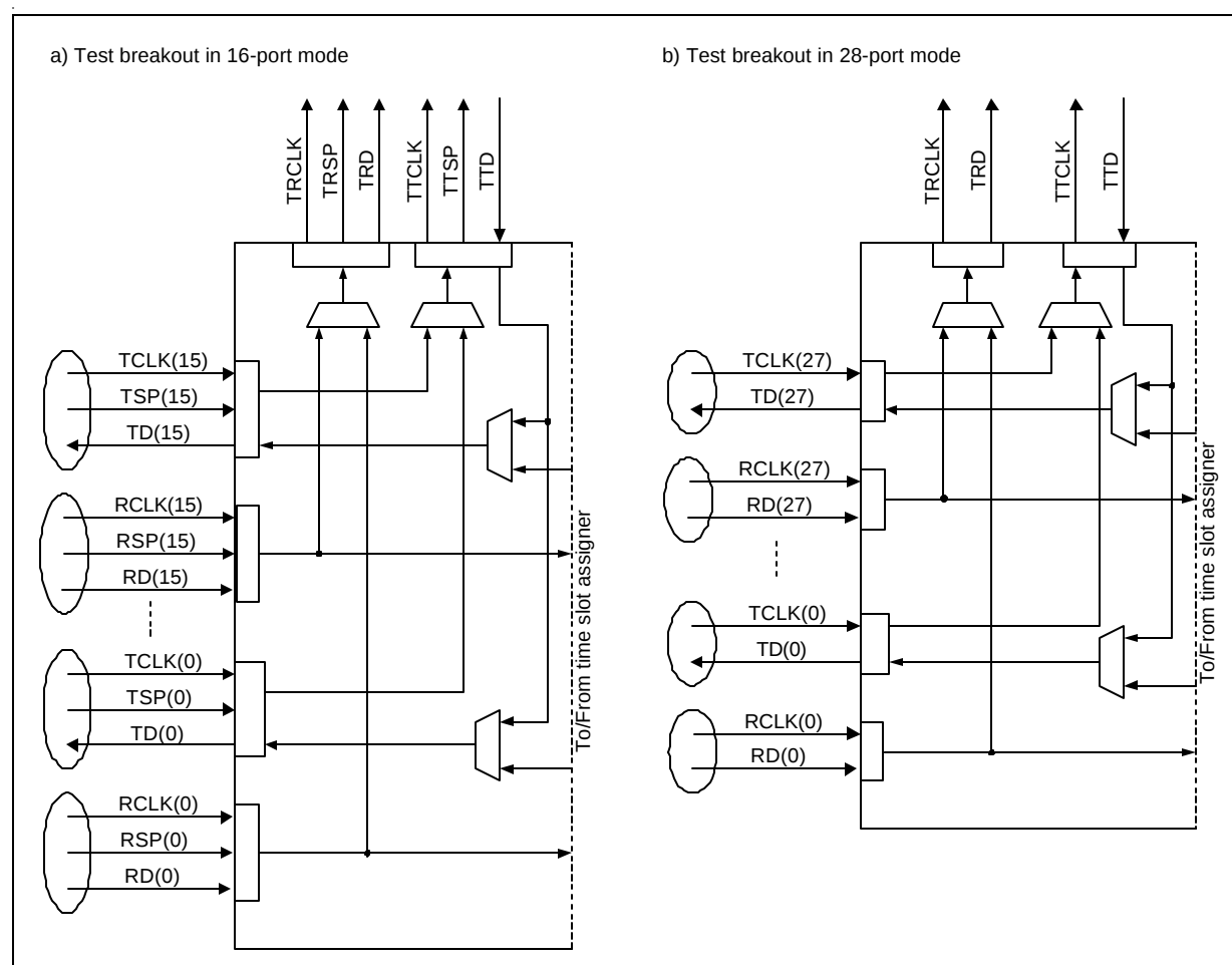
Figure 4-5 Test Breakout
