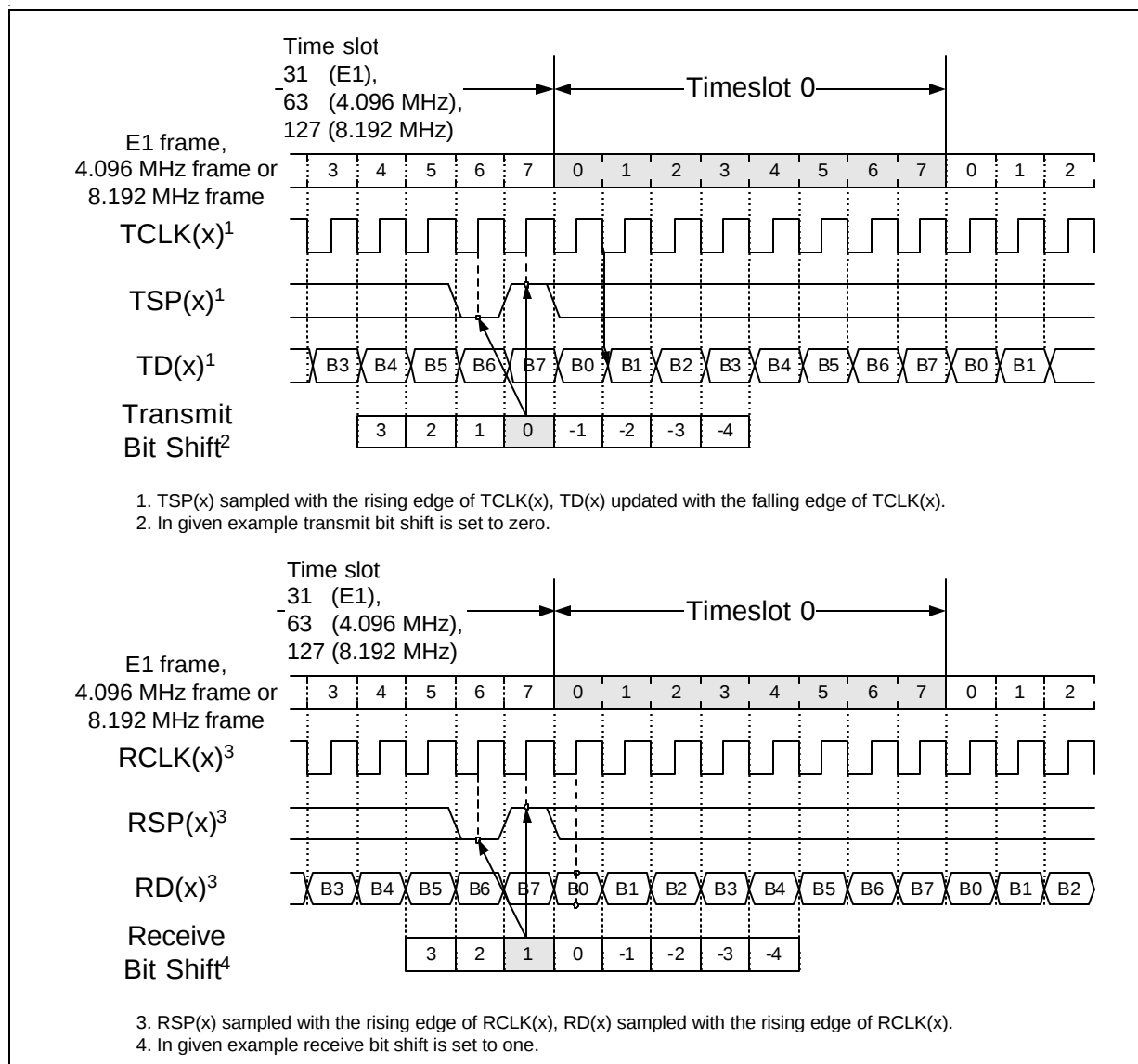
Figure 5-11 E1, 4.096 MHz and 8.192 MHz Interface Timing in 16-port mode
