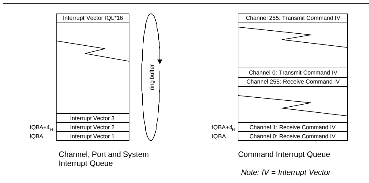
Figure 4-14 Interrupt Queue Structure in System Memory
