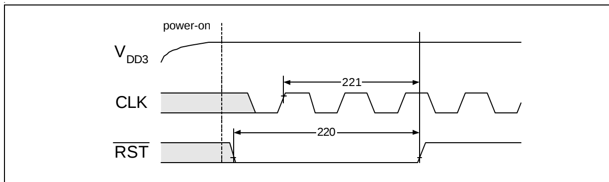
Figure 9-26 Reset Timing
