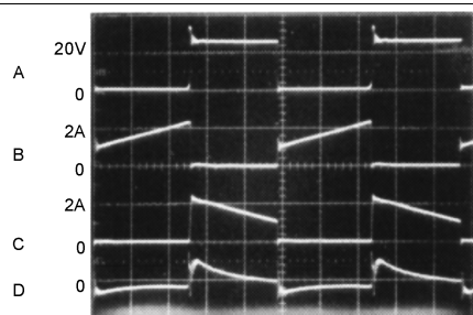
A: Switch Voltage, 20 V/div B: Switch Current, 2 A/div C: Output Rectifier Current, 2 A/div D: Output Ripple Voltage, 50 mV/div AC-Coupled Horizontal: 2 \mu s/div
