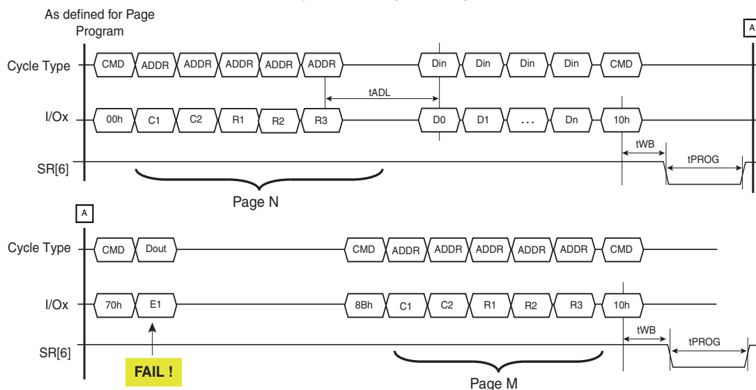
Figure 3.1 Page Reprogram
