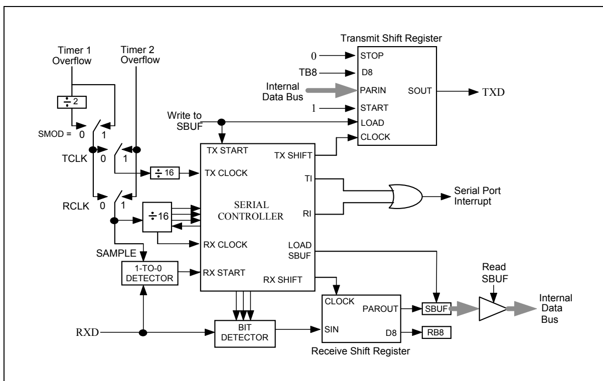
Figure 12-4 Serial Port Mode 3
