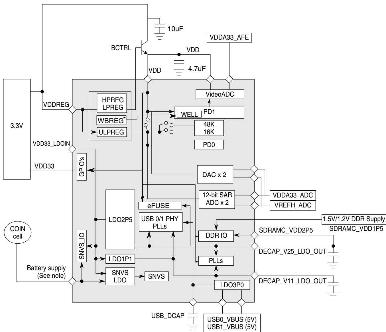
Figure 4. Power supply
