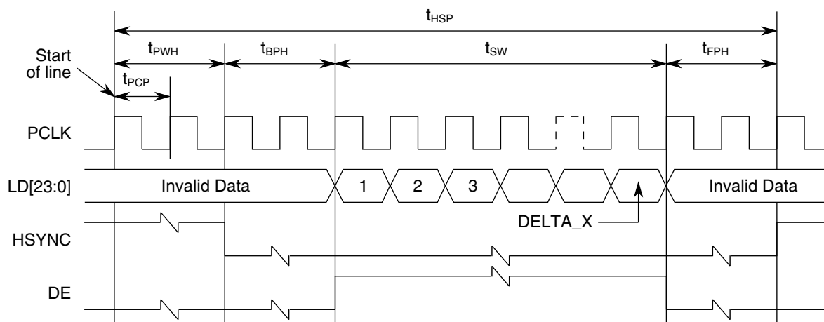
Figure 15. Horizontal sync timing
