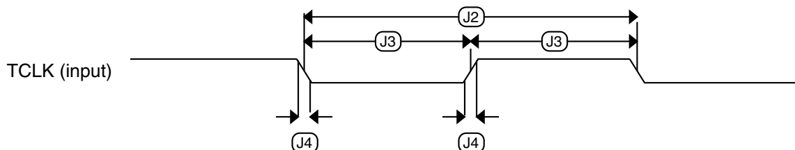
Figure 53. Test clock input timing
