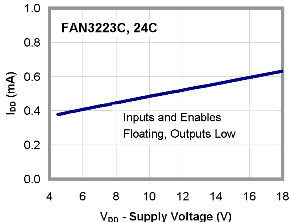
Figure 12. I_{DD} (Static) vs. Supply Voltage (Note 14)
